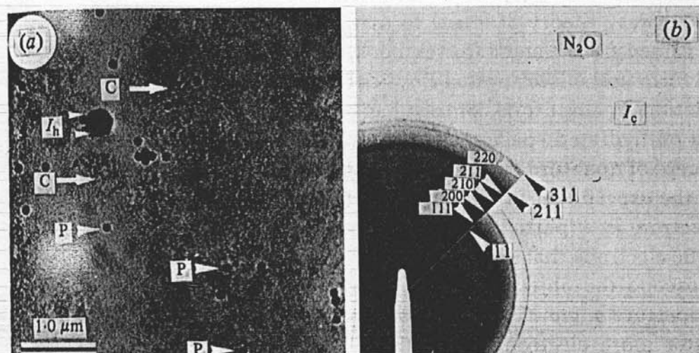
Fig. 38. Beam-induced formation of nitrous oxide crystals from a carbon-coated collodion film covered with a layer of cubic ice. The dose given is 4 \text{ ke/nm}^2 and the temperature is -160 \text{ }^\circ\text{C} . (a) Direct image. C, Crystals of \text{N}_2\text{O} ; P, polystyrene spheres; I_h , contaminating hexagonal ice crystal. (b) Electron diffractogram of the same field showing a powder diffractogram with the ring of cubic ice and \text{N}_2\text{O} . The (211) reflection of cubic ice I_c corresponds to 0.224 \text{ nm} . (From Dubochet et al. 1982a, with permission.)
