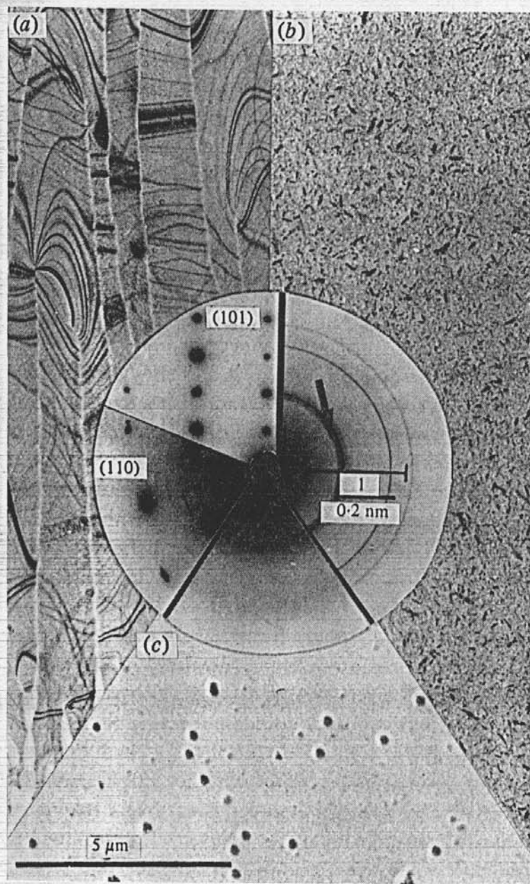
Fig. 5. Typical images and electron diffractograms of three forms of solid water observed in the electron microscope. The direct images and their diffractograms are all printed at the same scale. (a) Hexagonal ice obtained by rapid freezing of a water layer on a carbon film. The diffractograms, obtained from other specimens, show the (110) and (101) plane. (b) Cubic ice obtained by warming a layer of vitreous water obtained by condensation. The shoulder on the (111) reflection, possibly indicating the presence of a small amount of hexagonal ice, is marked by an arrow. (c) Vitreous water obtained in the microscope, by condensation of vapour on a cold carbon film supporting polystyrene spheres. The shadow effect demonstrates that the flux of water molecules was anisotropic. (From Dubochet et al. 1982c.)
