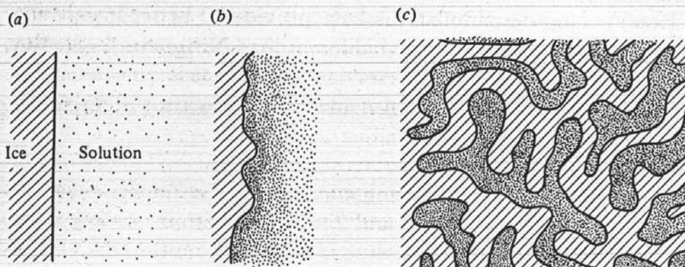
Fig. 10. Growth of a hexagonal ice crystal in an aqueous solution. Starting from a flat surface in a homogeneous solution (a), the rapid growth of the crystal makes the solute accumulate in front of the ice surface. This reduces the crystallization speed. Local statistical fluctuations in growth are amplified by the resistance of the concentrated solute layer (b). Finally, all the freezable volume may be filled by the ramified network of a single or a few crystals (c).
