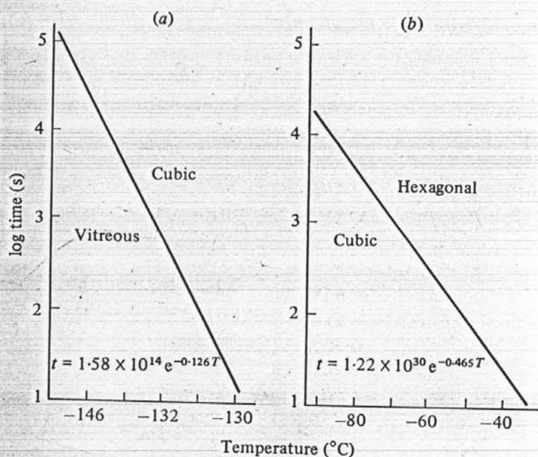
Fig. 6. Time t required, at the temperature T ( ^{\circ}\text{C} ), for the phase transition from (a) vitreous water to cubic ice and (b) cubic to hexagonal ice to take place (Dowell & Rinfret, 1960). Recent results suggest that curve (a) should be displaced by 10\text{--}20 ^{\circ}\text{C} towards the higher values (see text).
