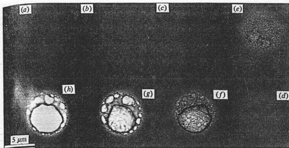
Fig. 37. Bubbling on a carbon-coated formvar film c. 10 \text{ nm} thick, covered with a layer of condensed vitreous water. Fields (a)–(h) correspond to irradiations by 5, 20, 40, 80, 120, 240, 340 and 450 \text{ ke/nm}^2 respectively. The total thickness of the specimen is 160 \text{ nm} .
