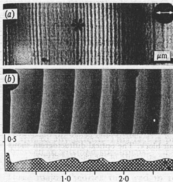
Fig. 18. Chatter in vitrified sections. (a) Solution of 40% bovine serum albumin. Two modes of vibration with periods of 0.2 and 4\ \mu\text{m} are superimposed. Sectioning temperature: -160^{\circ}\text{C} . Sectioning speed: 6\text{ mm/s} . Thickness: \geq 120\text{ nm} . (b) Saw tooth in a section of pure vitreous water. Sectioning speed: 0.2\text{ mm/s} . (c) Representation at the same scale of the thickness of the section shown in (b).
