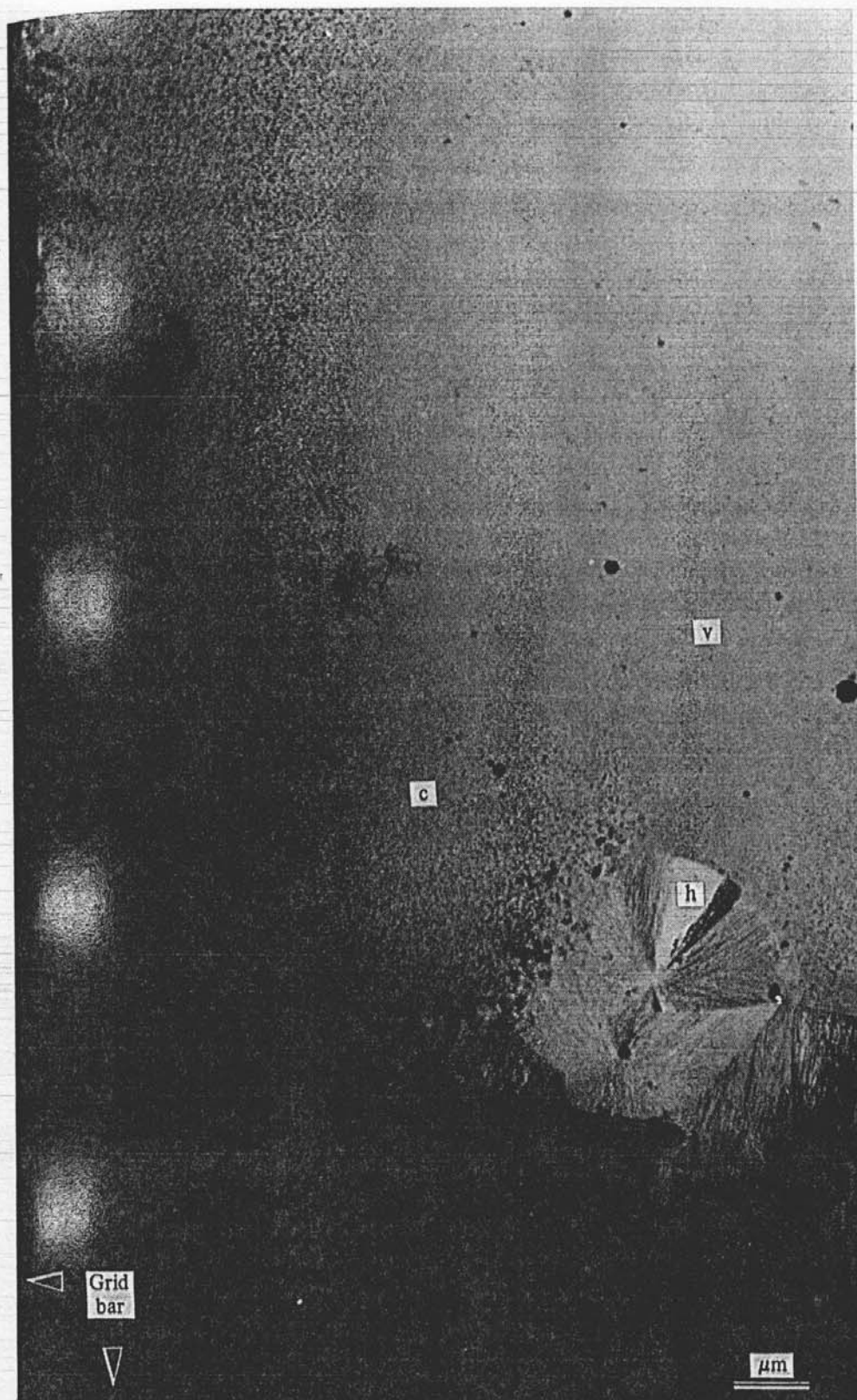
Fig. 48. Thin layer of nearly pure water in which hexagonal (h) and cubic (c) ice coexist with vitreous water (v). The thinnest region of the film is vitreous whereas the thicker regions, close to the grid bars, are crystallized.
