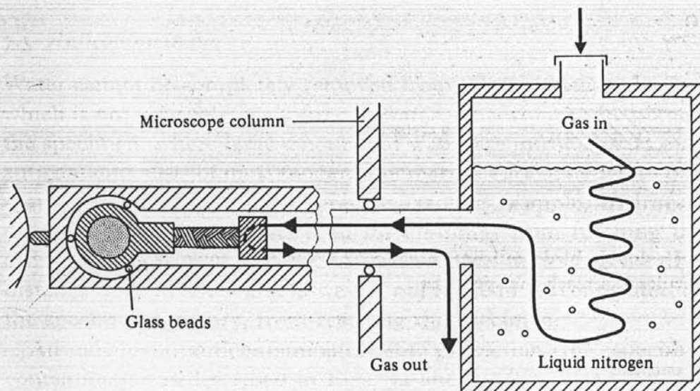
Fig. 36. Schematic view of the gas-cooled cryospecimen holder of the type Philips PW/6591. For a better representation in the drawing, the tip of the holder is rotated by 90^\circ in respect of the liquid-nitrogen recipient. For explanation, see text.
