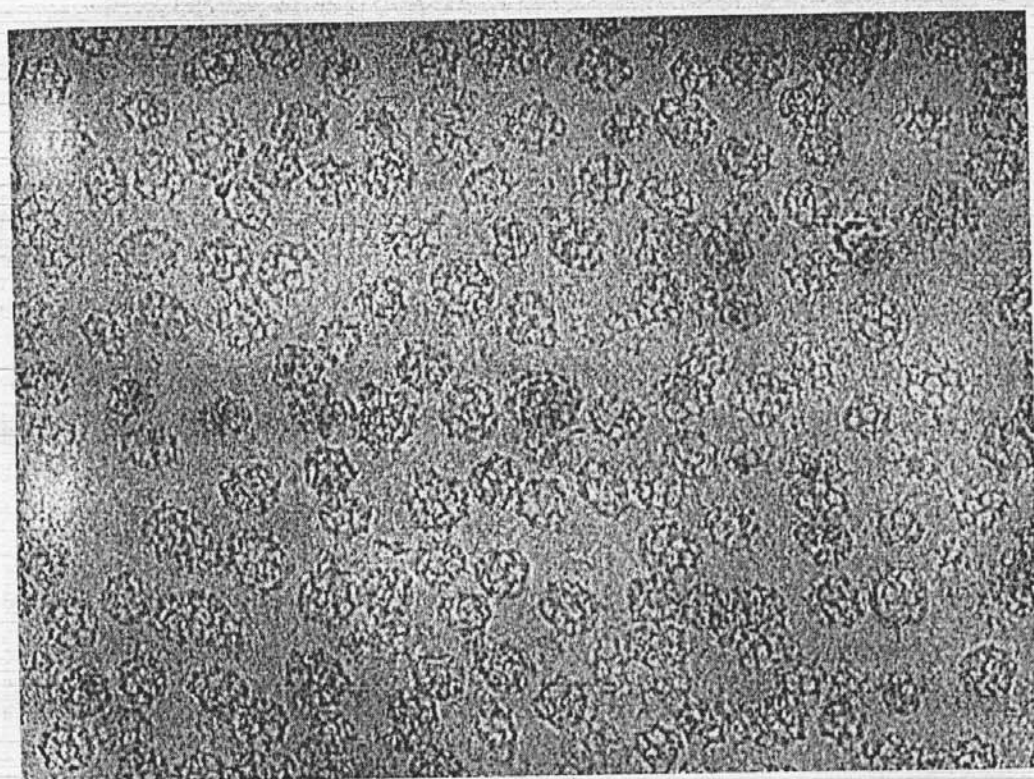
Fig. 59. Purified clathrin cages in vitreous ice. (Courtesy G. Vigers, Boulder, Colorado.)
