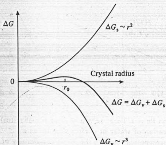
Fig. 8. Classical nucleation theory. The free energy, \Delta G , of a spherical ice crystal of radius r in water below 0^\circ\text{C} can be expressed as the sum of volume, \Delta G_v , and surface, \Delta G_s , contributions. Below r_0 the crystal is unstable.
