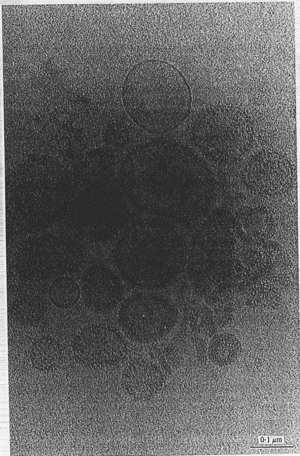
Fig. 55. Virosomes formed by lipid vesicles containing spike proteins of vesicular stomatitis virus (Material: courtesy K. Metsikkö, Heidelberg.)
