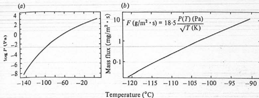
Fig. 7. (a) Vapour pressure P expressed in Pa ( 133 \text{ Pa} = 1 \text{ Torr} ; 10^5 \text{ Pa} = 1 \text{ bar} = 0.987 \text{ atm} ) as a function of the temperature in ^{\circ}\text{C} . (b) Evaporation of water in perfect vacuum as a function of the temperature in ^{\circ}\text{C} . One \text{mg}/\text{m}^2 corresponds to 1 \text{ nm} thickness at a density of 1 \text{ g}/\text{cm}^3 .
