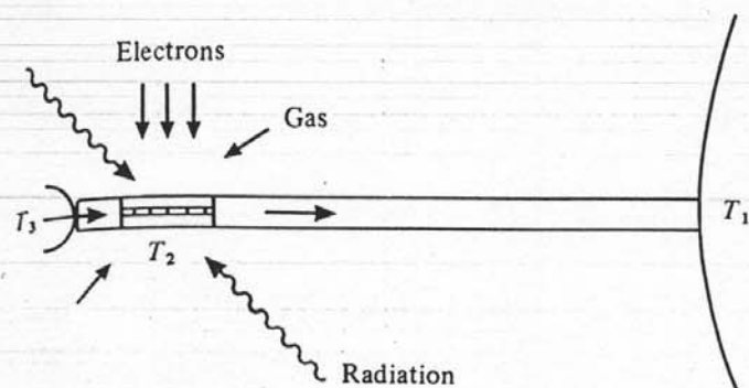
Fig. 30. Schematic representation of a side-entry cryospecimen holder cooled by conduction in a metal rod. The temperature T_2 of the specimen results from the balance between the cooling of the liquid nitrogen at temperature T_1 , -196^\circ\text{C} , and the heating from the warm surrounding, acting by direct contact with surfaces at room temperature, T_3 , by gas conduction, by radiation and by the energy brought with the electron beam.
