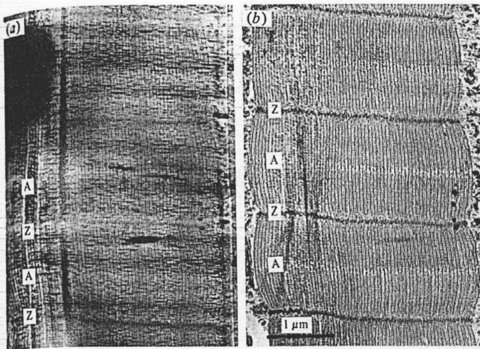
Fig. 16. Longitudinal cryosection of glycerinated insect flight muscle washed in 20% sucrose buffer. This region of the sample was not vitrified, but water was crystallized into cubic ice. (a) Fully hydrated section. (b) Same region as in (a) after freeze drying in the microscope. A and Z: A and Z bands. (From Dubochet & McDowall, 1984.)
