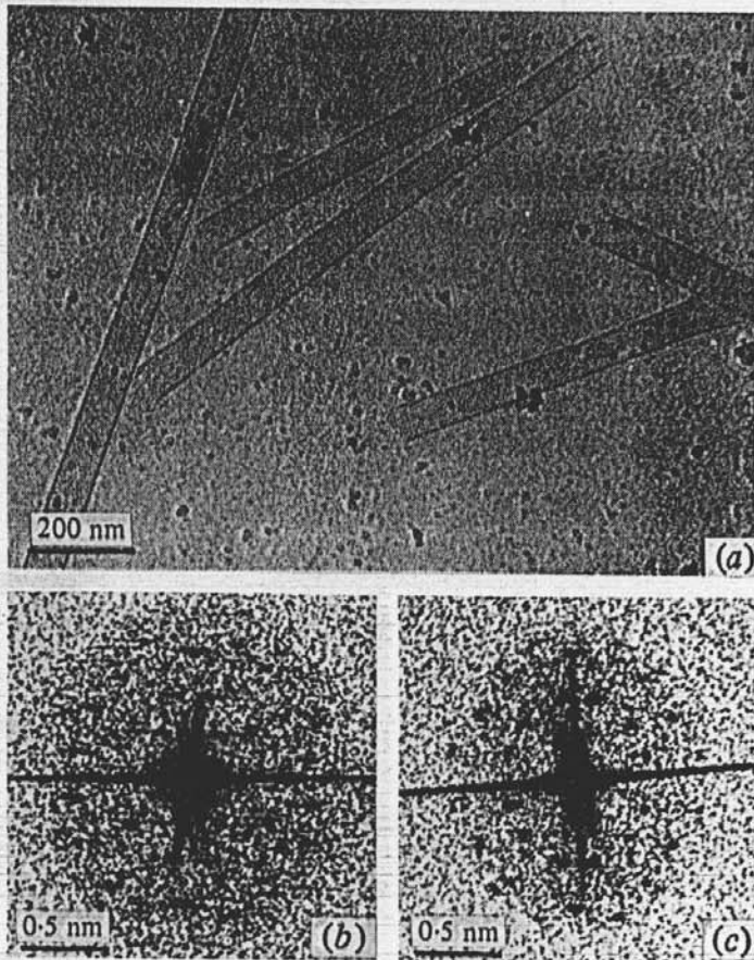
Fig. 25. Polyheads of the T 4 bacteriophage. (a) Prepared in a c. 100 nm thick layer of vitrified solution. Two particles are flattened at the point where they are superimposed. (b) Optical diffractogram of a particle shown in (a). It is characteristic for a cylindrical particle. (c) Optical diffractogram of a particle embedded in a vitrified layer, much thinner than the particle diameter. It is characteristic of a flattened particle. (From Lepault (1985), with permission.)
