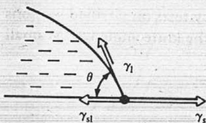
Fig. 22. Interfacial tension of a liquid on a solid. The Young condition states that, at equilibrium, the surface tension of the solid, \gamma_s , of the liquid, \gamma_l and of the interfacial tension, \gamma_{sl} , are related by the relation \gamma_{sl} + \gamma_l \cos \theta = \gamma_s , in which \theta is the wetting angle.
