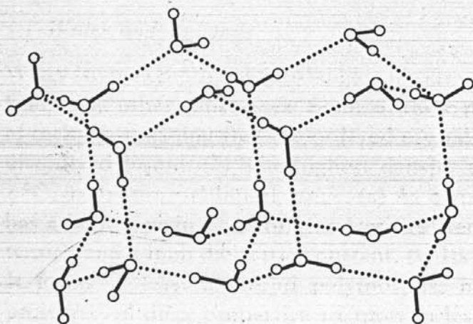
Fig. 2. Schematic view of a small part of a hexagonal ice crystal.
