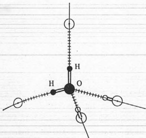
Fig. 1. Tetrahedral structure of the fully hydrogen-bonded water molecule.
