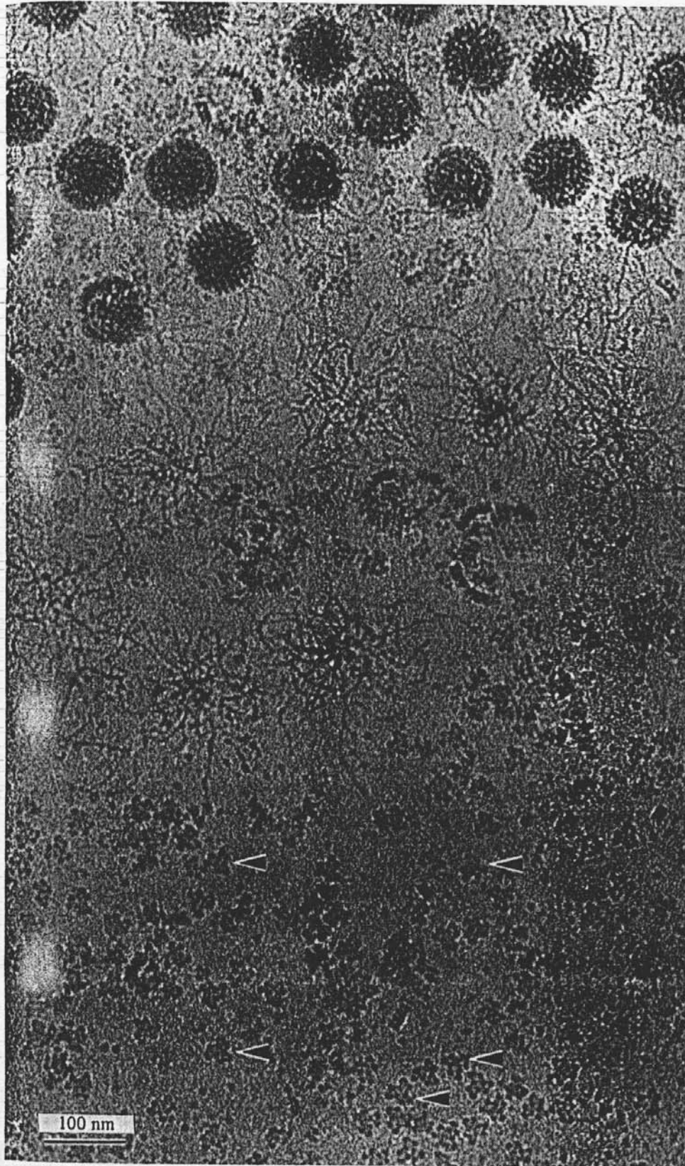
Fig. 26. Thin vitrified layer of a solution of partially disrupted adenovirus. Many groups of nine (G 9 ) are visible; some have been marked by an arrow. (From Dubochet et al. 1985.)
