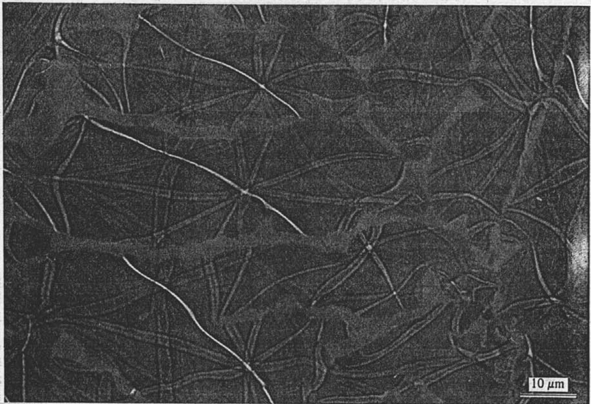
Fig. 47. Thin crystal of hexagonal ice obtained by freezing of a water drop while it was spreading on the partially hydrophilic carbon support. Bend contours due to Bragg reflexions of the deformed crystal are clearly seen.
