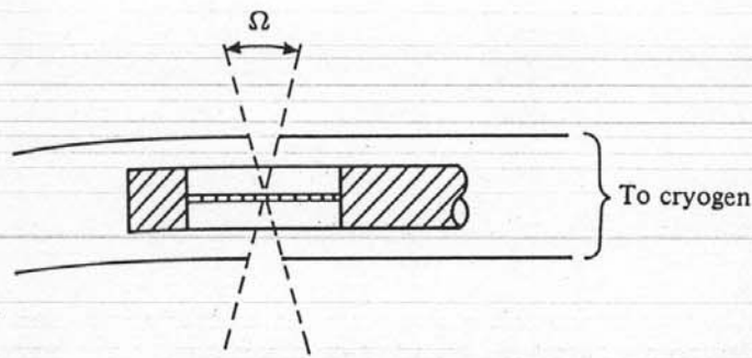
Fig. 34. Principle of a double-blade anticontaminator. \Omega is the solid angle in which contaminating molecules can reach the specimen.
