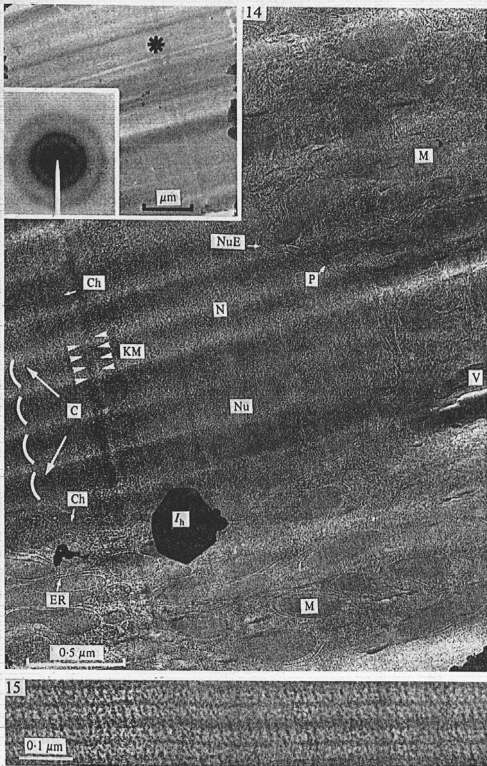
Fig. 14. Section from an untreated fragment of rat liver, vitrified by projection on a cold metal block. Sectioning temperature: -160^{\circ}\text{C} . Thickness: 180 nm. N, nucleus; Nu, nucleolus; NuE, nuclear envelope; P, nuclear pore; Ch, chromatin; M, mitochondria; ER, endoplasmic reticulum with ribosomes; V, vacuole; I_h : contaminating hexagonal ice crystals; KM, knife marks; C, chatter. Insert: section from a block of vitreous ice with its electron diffractogram. The block was obtained by condensation of water vapour at -10^{-1} Pa for 2 hours on a specimen holder kept at liquid nitrogen temperature. Sectioning temperature: -160^{\circ}\text{C} . The thickness at the point marked by a star is 120 nm. The first separated ring in the diffractogram corresponds to 0.37 nm (From: McDowall et al. (1983), with permission.) Fig. 15. Longitudinal cryosection in a vitrified unfixed fibril of glycerinated insect flight muscle in the relaxed state. Section thickness: 80 nm. (From McDowall et al. (1984), with permission.)
