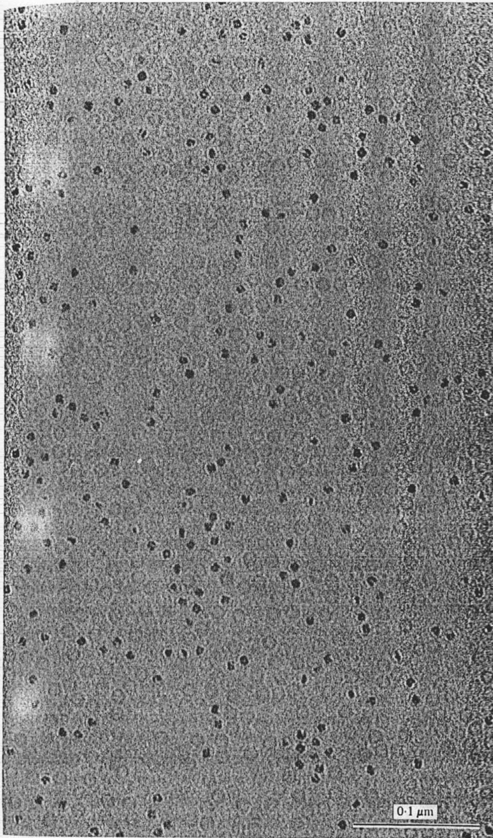
Fig. 54. Ferritin and apoferritin prepared by the perforated-film method. (Material: courtesy W. H. Massover, Newark.)
