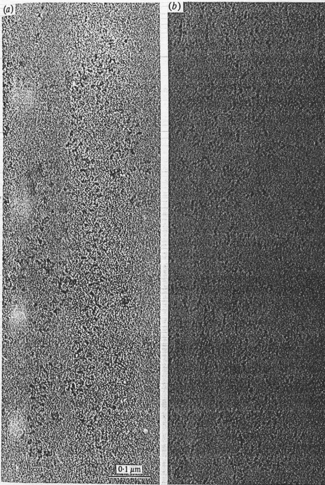
Fig. 56. (a) Chicken erythrocyte chromatin prepared by the perforated-grid method in 10 mM-NaCl. The individual nucleosomes are clearly visible along the zig-zaging filaments. (b) Turnip yellow mosaic virus RNA prepared by the perforated-film method in 125 mM-NaCl. (Material: courtesy J. Witz, Strasbourg.)
